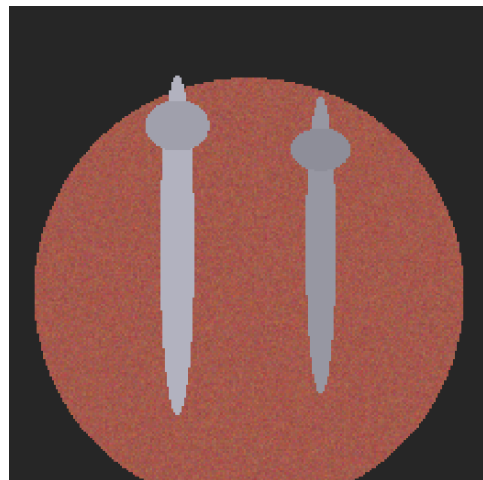
(e) Segmentation
